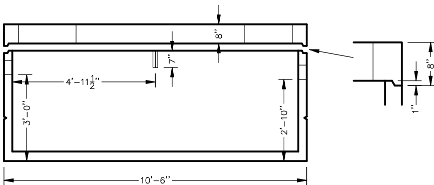
BASE: SIDE VIEW
