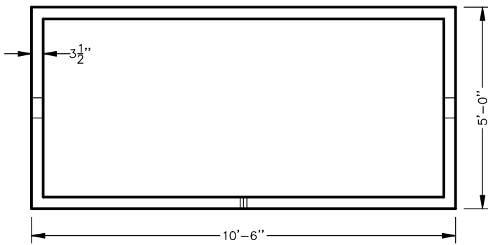
BASE: TOP VIEW
